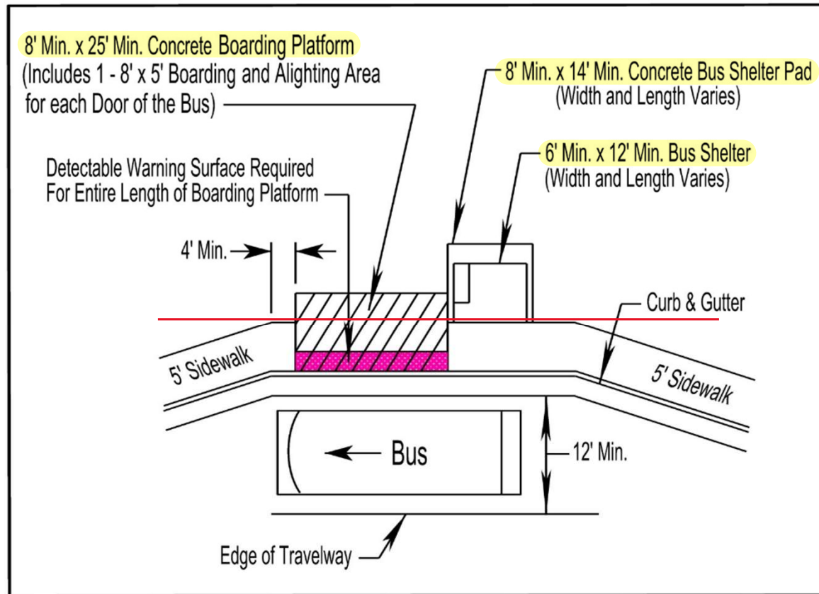
FIGURE A(1)- 48 ELEMENTS AND DIMENSIONS ASSOCIATED WITH BUS (TRANSIT) STOPS
